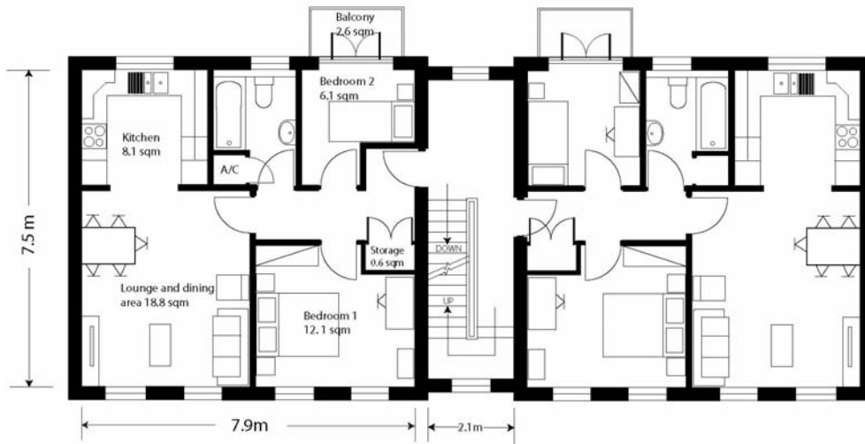
Figure 9.12 Volume house builder typical first floor flat layout, Gross Internal Floor Area 59 sq metres
