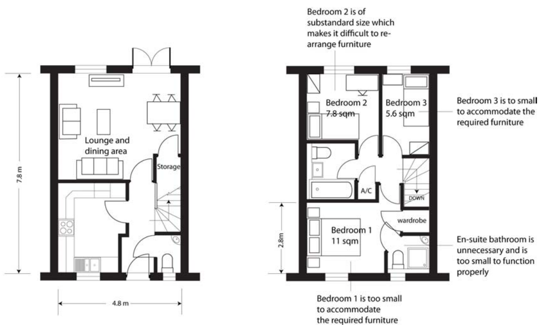
Figure 9.6 Typical volume house builder 3 bedroom house type. Gross internal floor area 74 square metres
