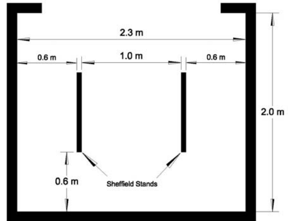
Figure 6.27 Internal dimensions of a communal cycle store
