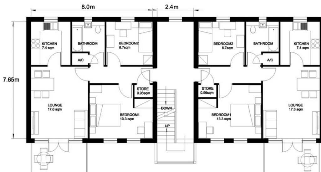
Figure 9.13 An example of first floor flat layout which meets the standards, Gross Internal Floor Area 61 sq metres
