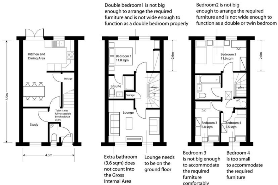
Figure 9.9 Typical volume house builder 4 bedroom townhouse type, Gross Internal Floor Area 106 sq metres.
