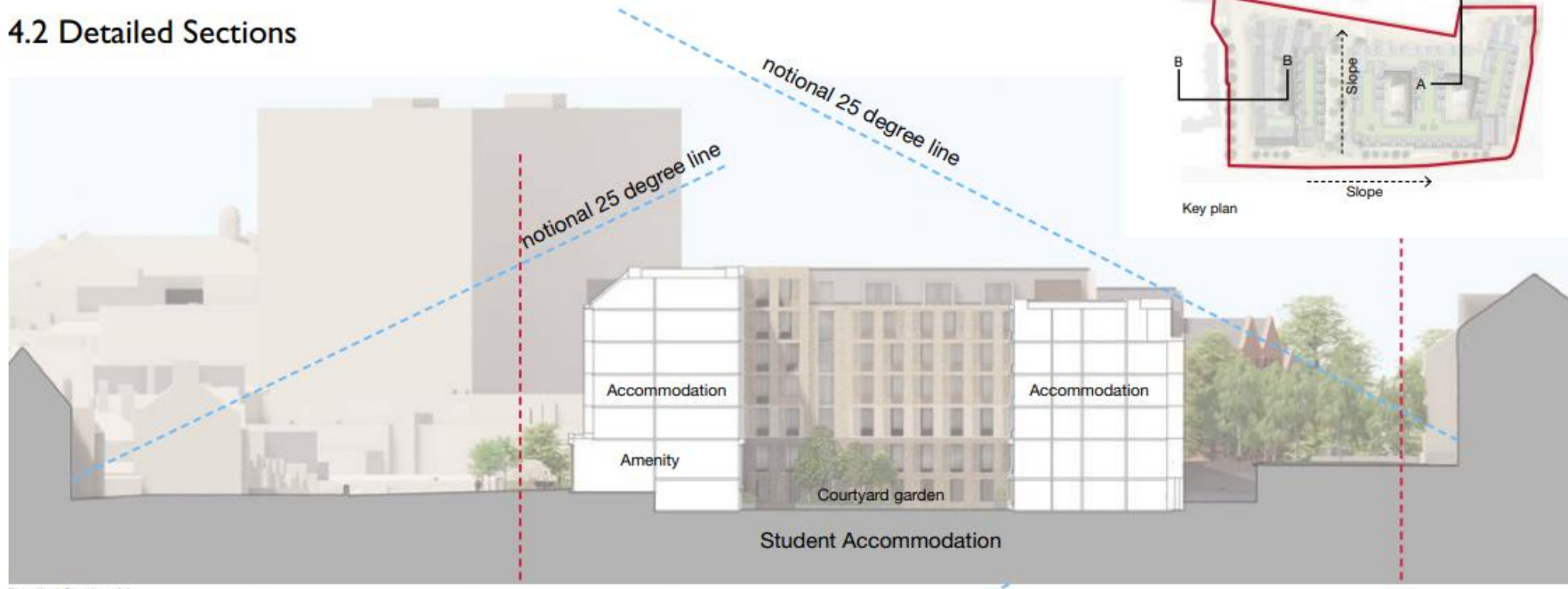
Detailed Section AA
