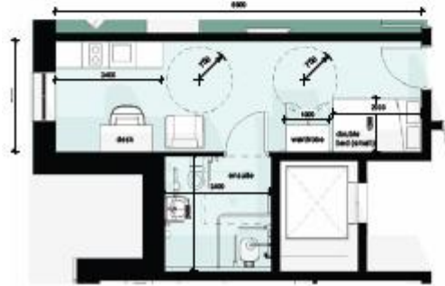
Co - Living Typical Accessible Studio
