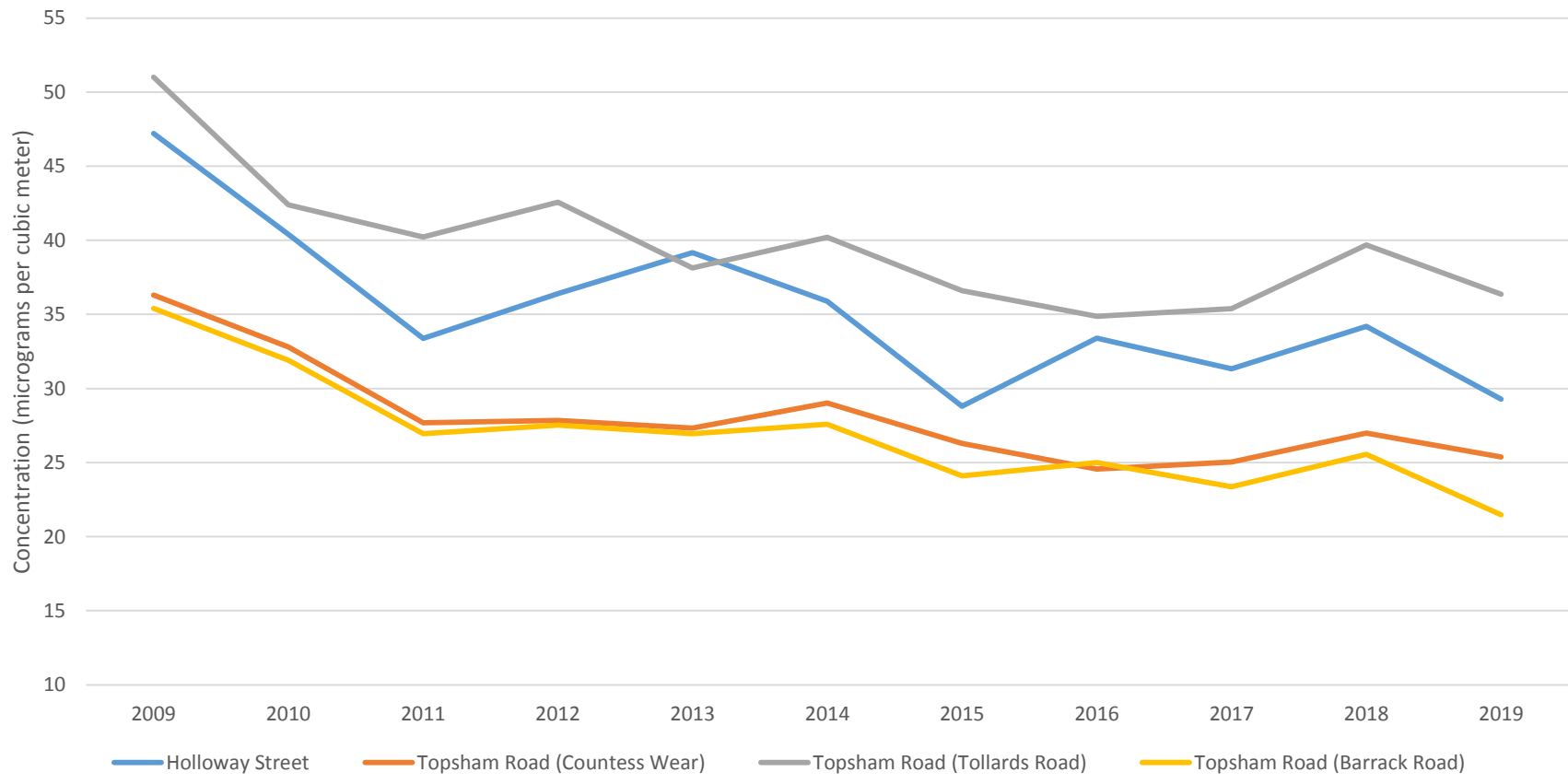
Nitrogen Dioxide Concentrations at Monitoring Points within the AQMA along the Topsham Corridor since 2009
