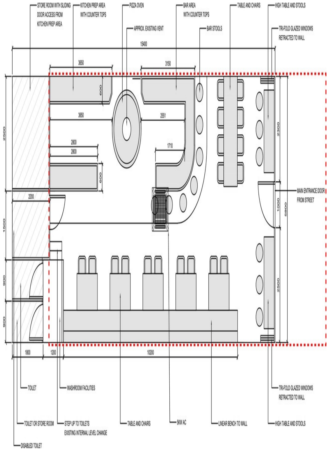
Existing: Floor Plan Scale: 1:75
